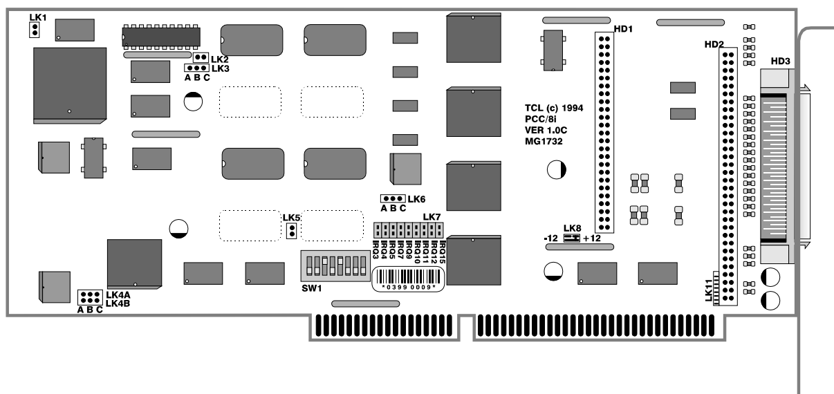
DataServer-8 Controller card (Prod. No. 210)
