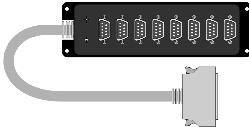
DataServer-8 RS232 Distribution Cable 9-Way D-Type Male (Part No. 9511) DataServer-8 RS422 Distribution Cable 9-Way D-Type Female (Part No. 9521)
